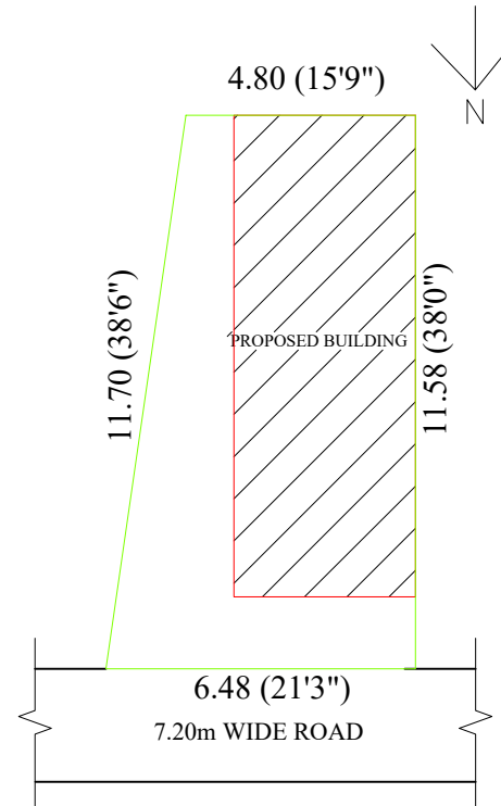
SITE PLAN
