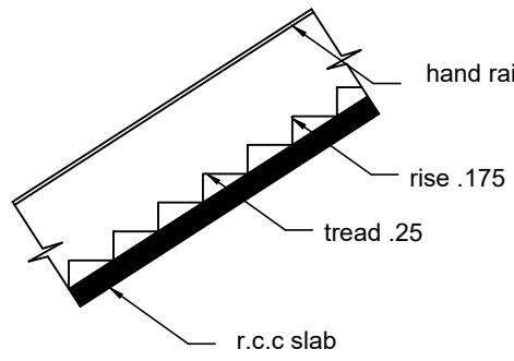
STAIR
