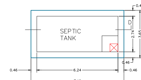
PLAN OF SEPTIC TANK SCALE 1"=2'0"
