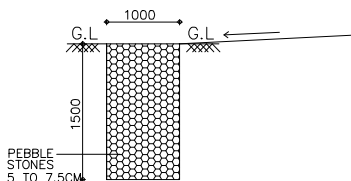
SECTION OF PEBBLE TRENCH SCALE : 1 : = 100
