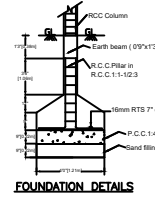
FOUNDATION DETAILS
