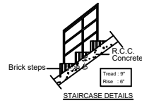
STAIRCASE DETAILS
