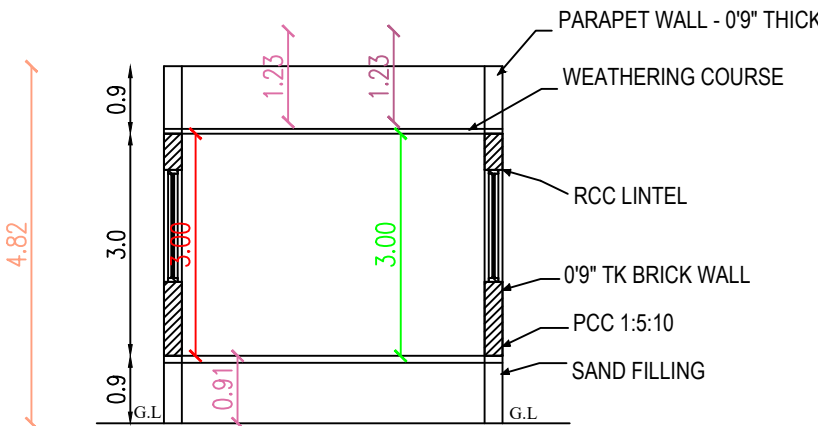
SECTION CUTTING XX
