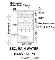
SCALE 1" = 8'0"
