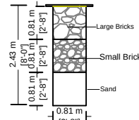
SECTION OF RAIN WATER COLLECTION PITS (NTS)
