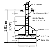
FOUNDATION DETAILS
