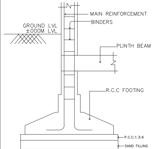
SCALE : 1" = 2'-0"
