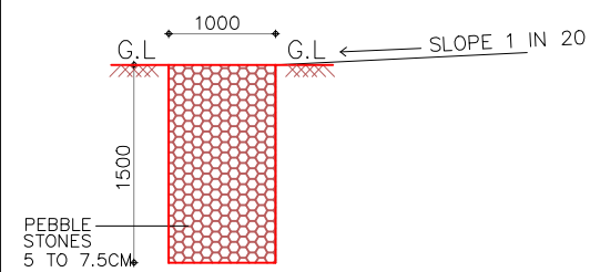
SUMP DETAIL
