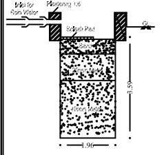
RAIN WATER PERCOLATION PIT
