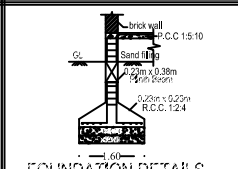
FOUNDATION DETAILS
