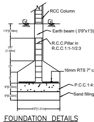
FOUNDATION DETAILS
