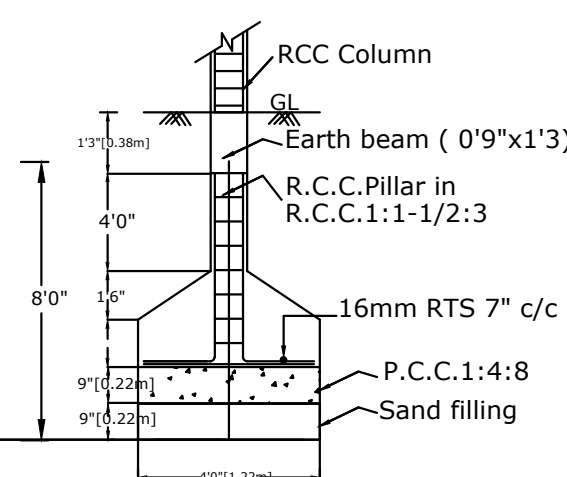
FOUNDATION DETAILS
