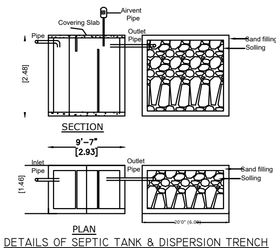
DETAILS OF SEPTIC TANK & DISPERSION TRENCH
