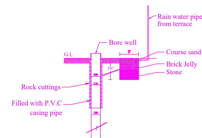
RAIN WATER HARVESTING DETAIL
