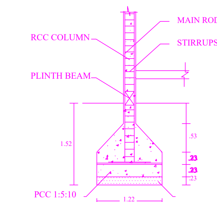
COLUMN DETAILS
