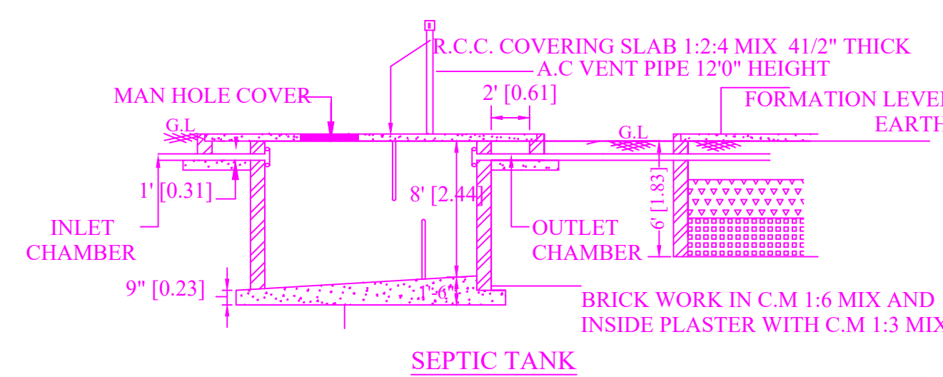
SEPTIC TANK
