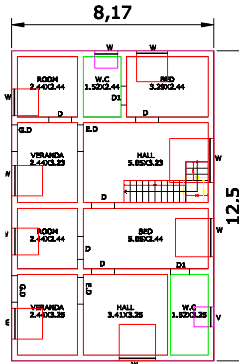
FIRST FLOOR PLAN RESIDENTIAL
