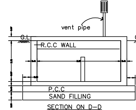
SECTION ON D-
