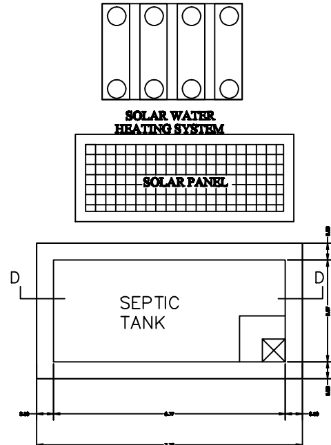
PLAN OF SEPTIC TANK SCALE 1"=2'0"
