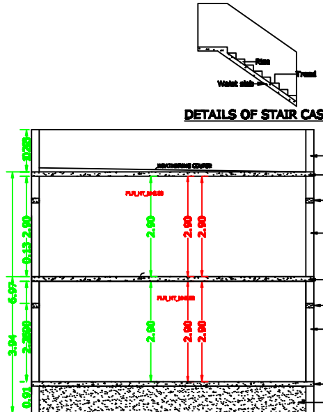
SECTION ON A-A
