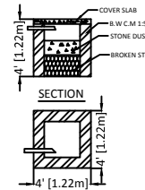
TRAIL PIT PLAN
