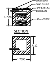
RAIN WATER HARVESTING PLAN
