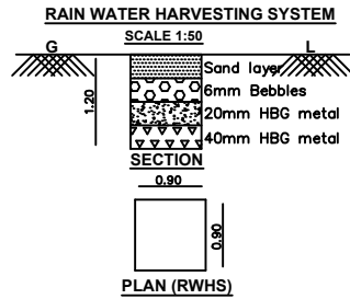
PLAN (RWHS)
