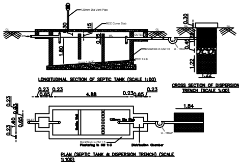
PLAN (SEPTIC TANK & DISPERSION TRENCH) (SCALE 1:100)
