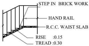
STAIR DETAILS
