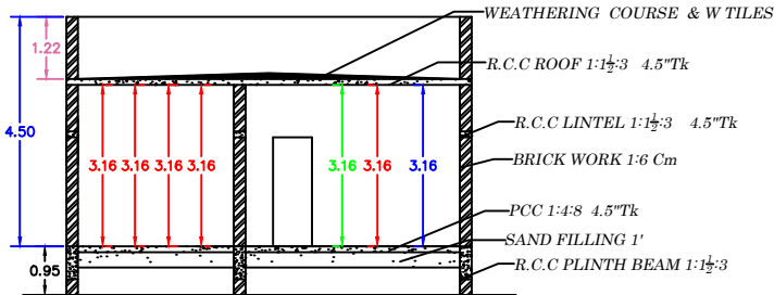
CUT SECTION AA'
