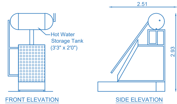
SOLAR WATER HEATING SYSTEM Not For Scale
