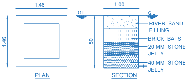
RAIN WATER HARVESTION Not For Scale
