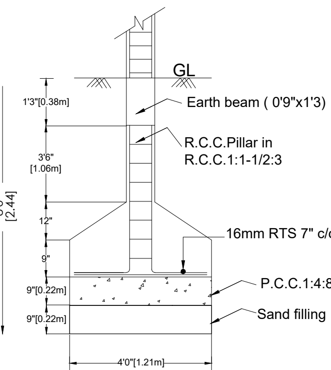
FOUNDATION DETAILS
