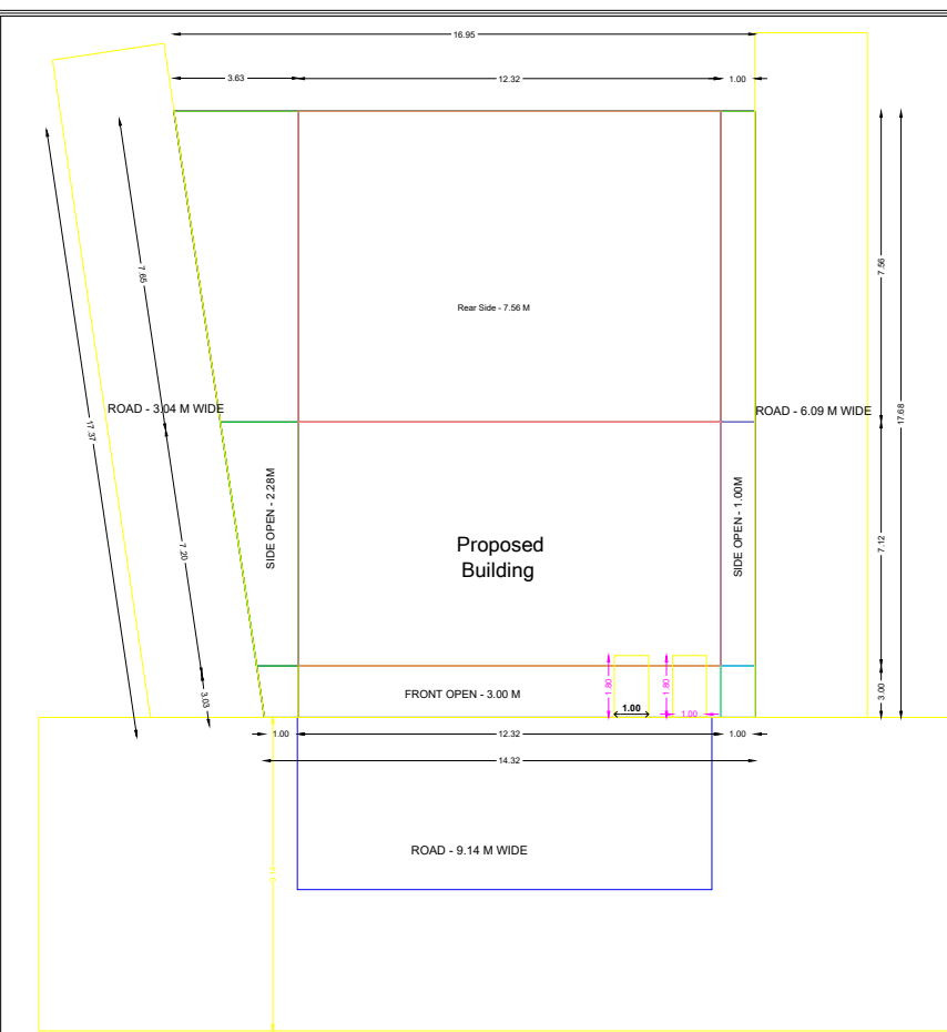
SITE BOUNDARY & PROPOSED SKETCH
