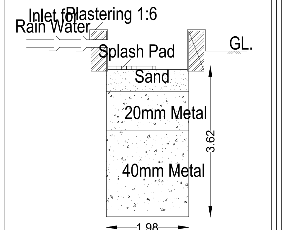
RAIN WATER PERCOLATION PIT
