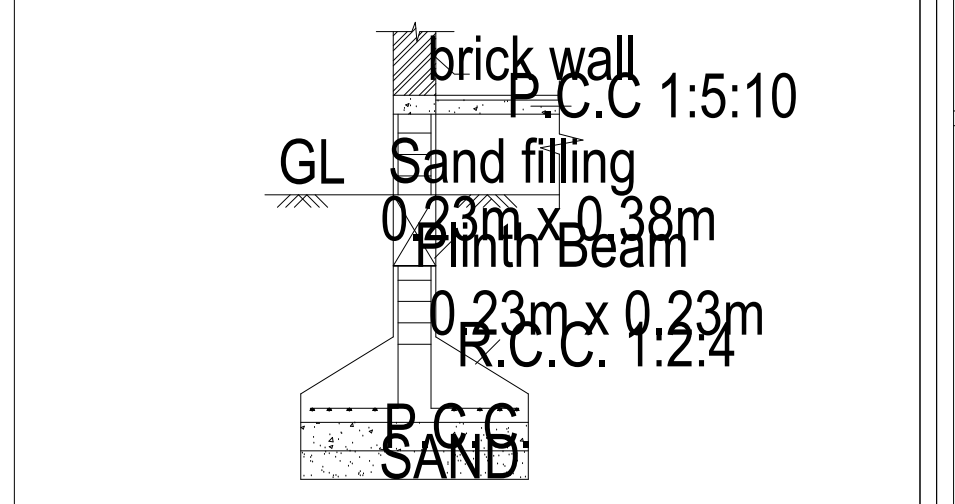
FOUNDATION DETAILS
