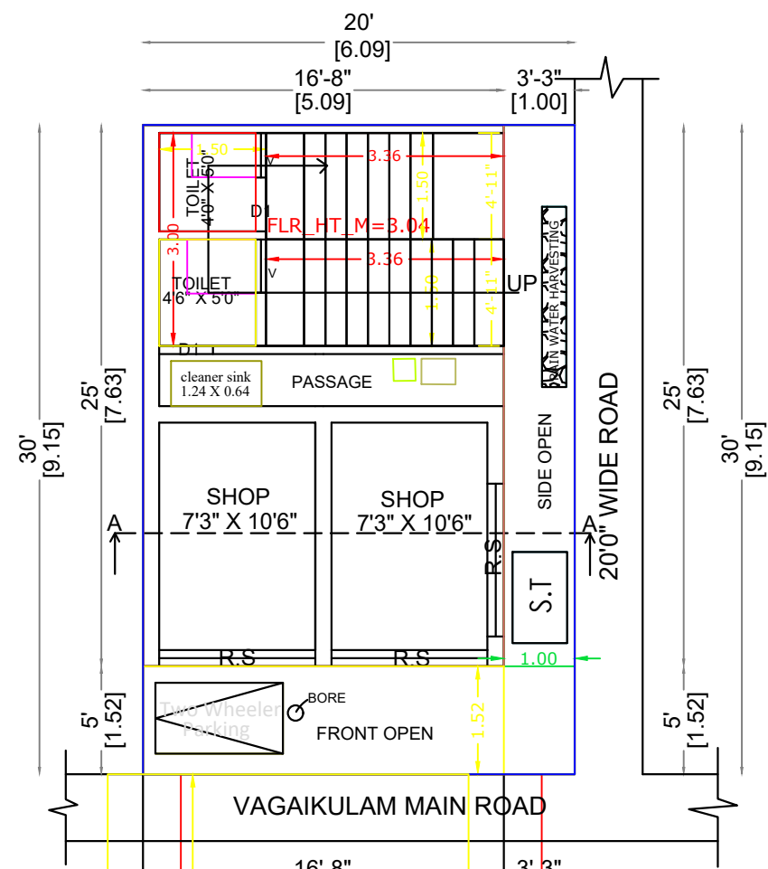
EXG.GROUND FLOOR PLAN
