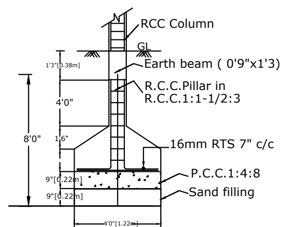
FOUNDATION DETAILS
