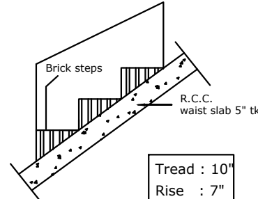
STAIRCASE DETAILS-nts
