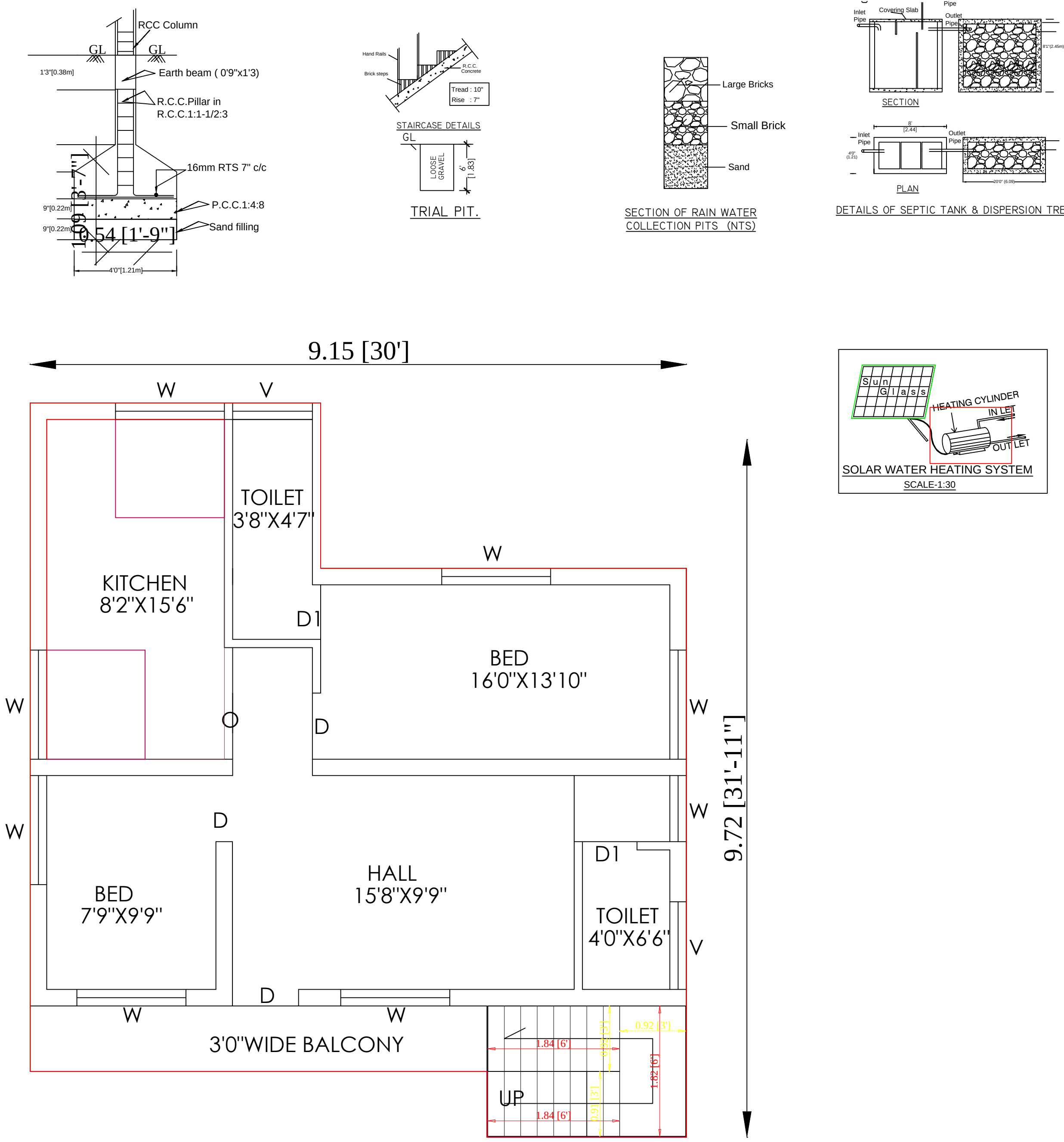
PRO.FIRST FLOOR PLAN
