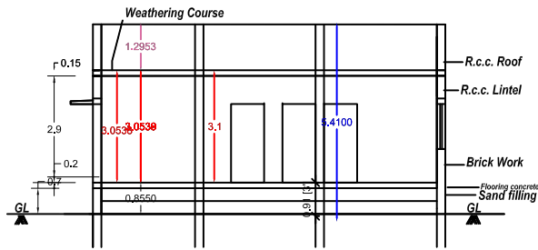
SECTION- BB
