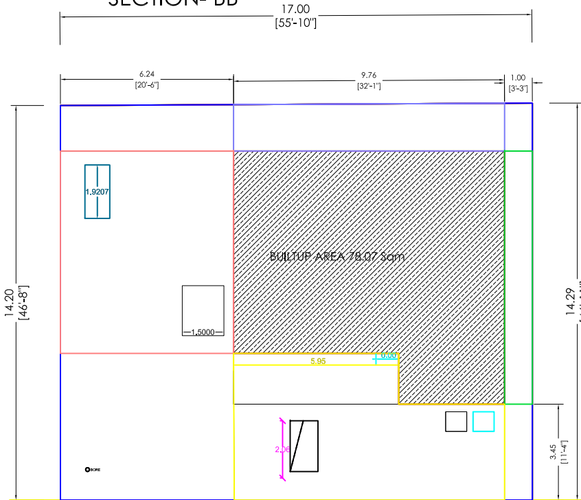
20'0" WIDE ROAD GROUND FLOOR PLAN PROPOSED
