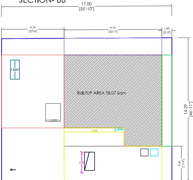
SECTION- BB
