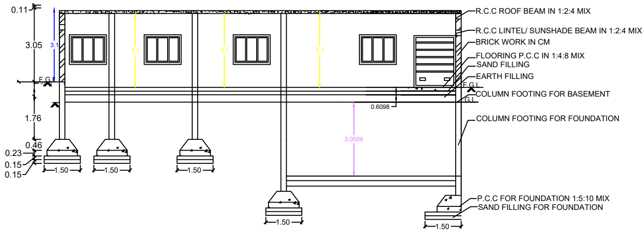
SECTION ON-AA
