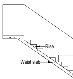
DETAILS OF STAIR CASE
