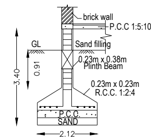
FOUNDATION DETAILS
