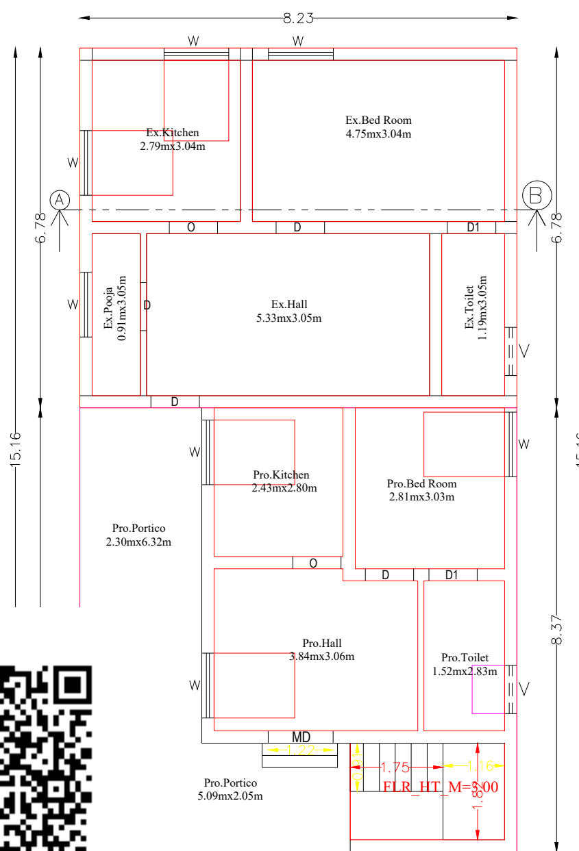
EXISTING GROUND FLOOR & PROPOSED GROUND FLOOR
