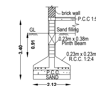
FOUNDATION DETAILS
