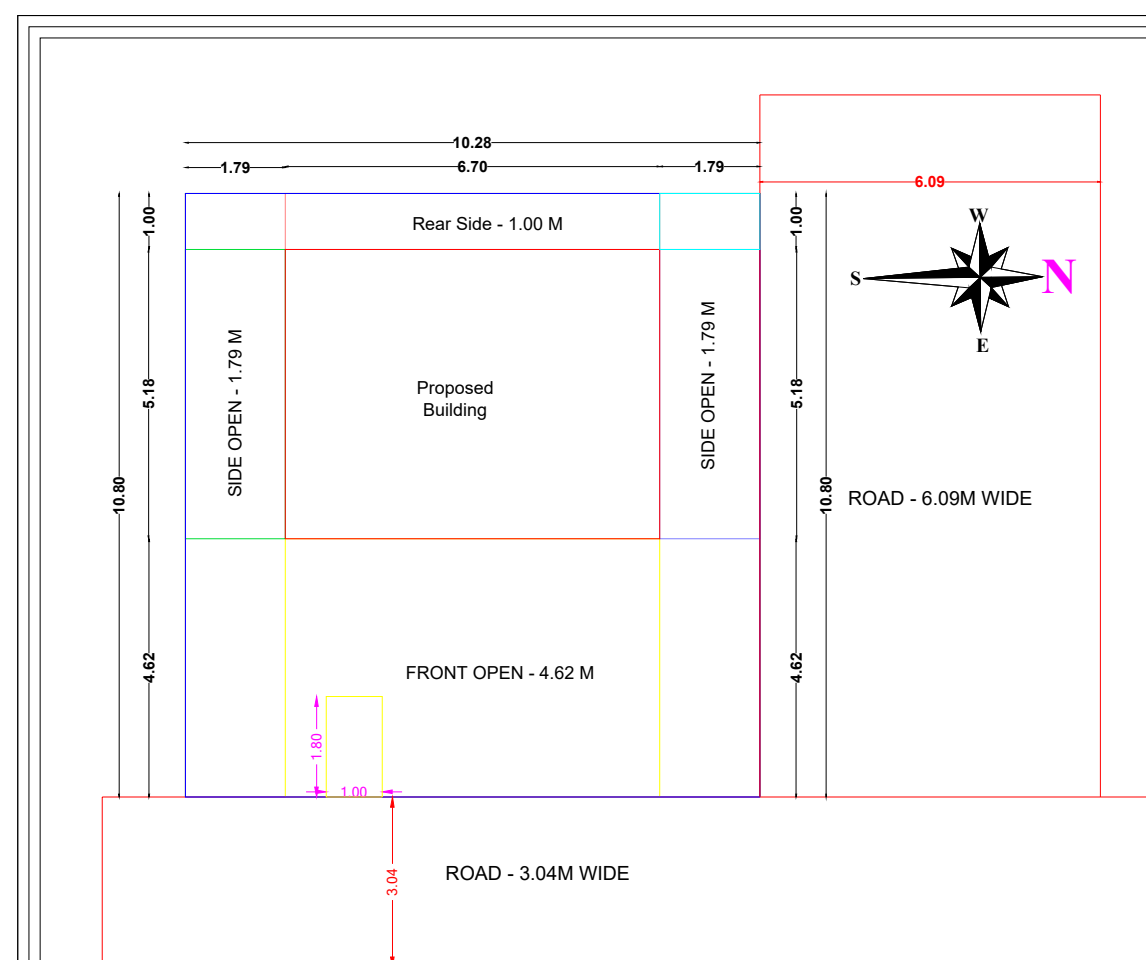
SITE BOUNDARY & PROPOSED SKETCH :
