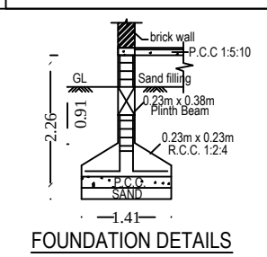
FOUNDATION DETAILS
