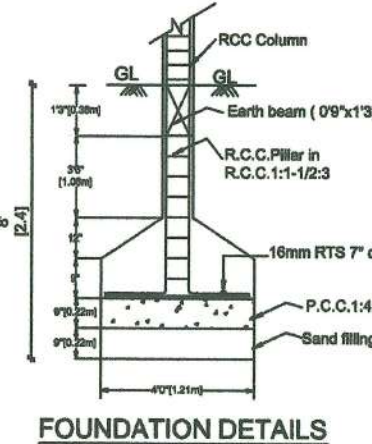
FOUNDATION DETAILS
