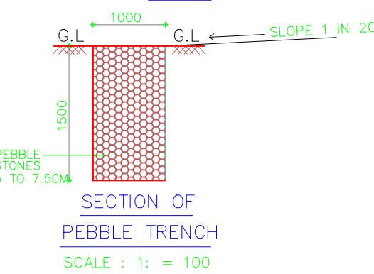
SECTION OF PEBBLE TRENCH SCALE : 1: = 100
