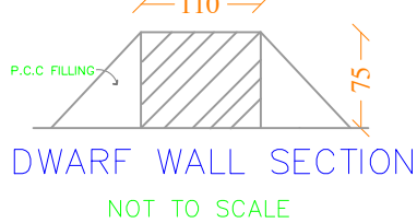
DWARF WALL SECTION NOT TO SCALE
