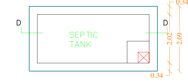
PLAN OF SEPTIC TANK SCALE 1"=2'0"
