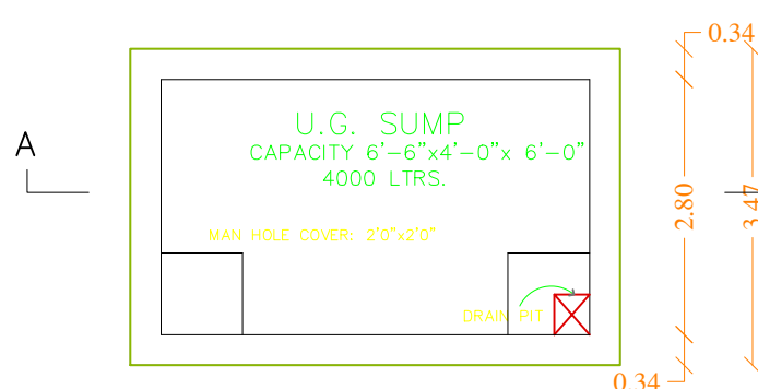
U.G. SUMP CAPACITY 6'-6"x4'-0"x 6'-0" 4000 LTRS.
