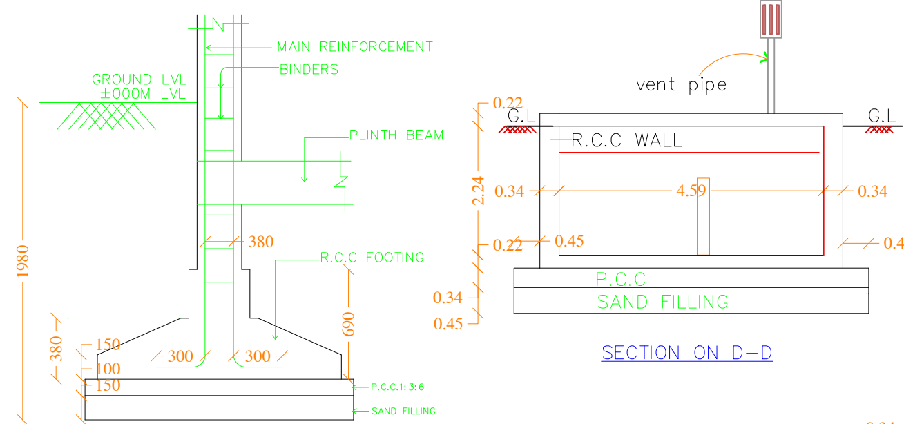
TYPICAL SECTION OF R.C.C COLUMN FOUNDATION SCALE : 1" = 2'-0"
