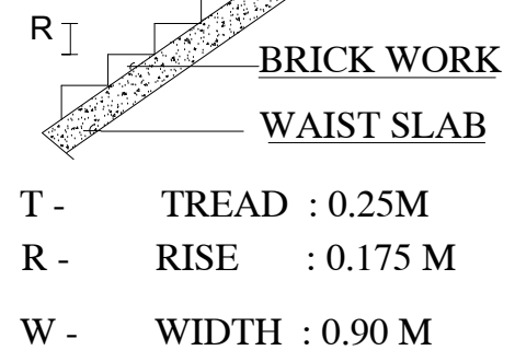
STAIRCASE DETAILS
