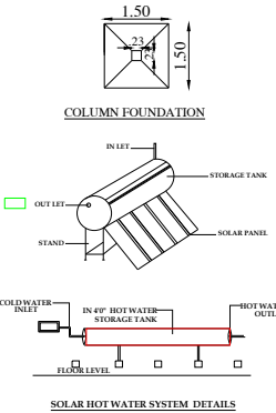
SOLAR HOT WATER SYSTEM DETAILS
