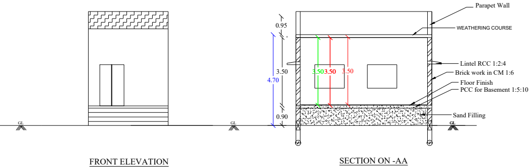
FRONT ELEVATION
