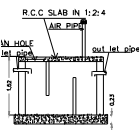
SEPTIC TANK SECTION
