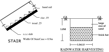
RAINWATER HARVESTING
