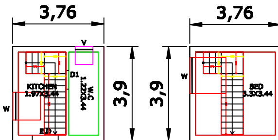
GROUND FLOOR PLAN FIRST FLOOR PLAN
