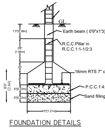
FOUNDATION DETAILS
