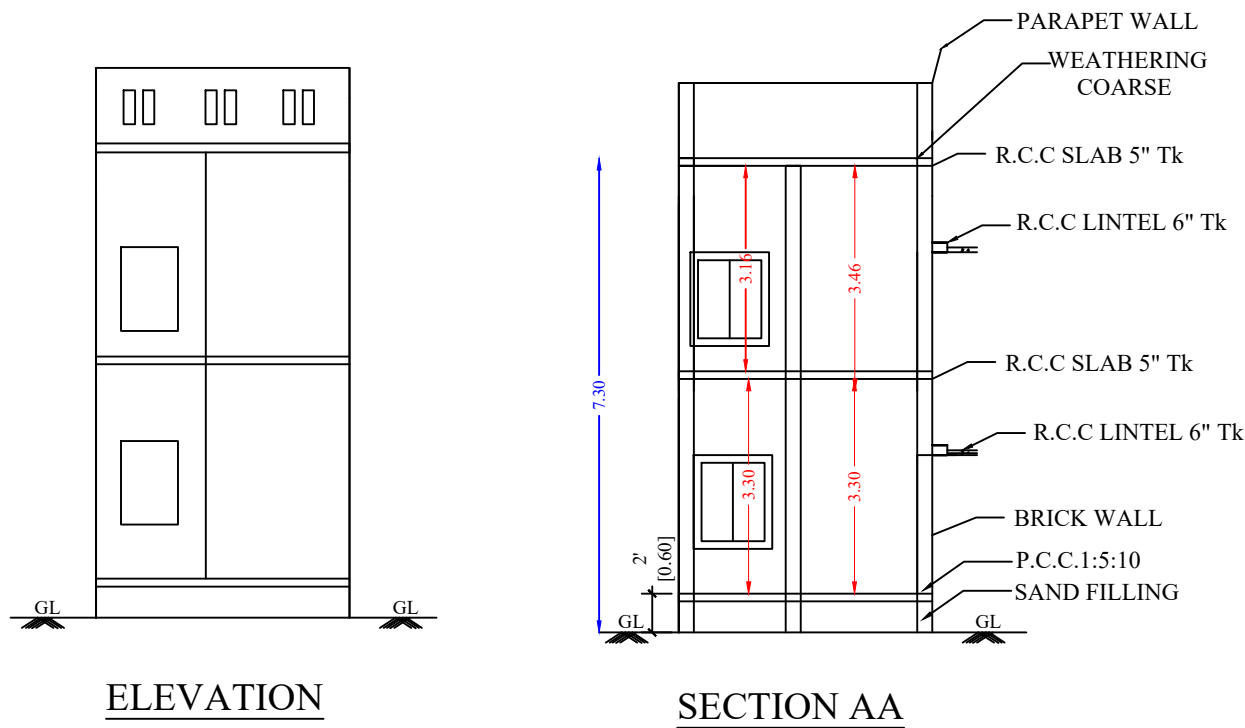
SECTION AA
