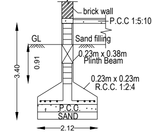
FOUNDATION DETAILS
