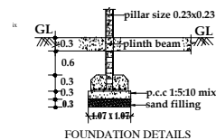
FOUNDATION DETAILS
