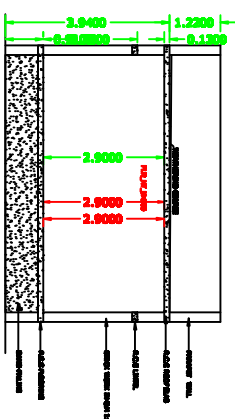
SECTION ON A-A
