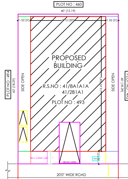
SITE PLAN
