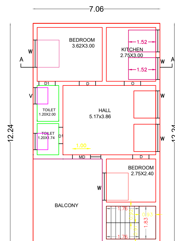
7.00 PROPOSED FIRST FLOOR PLAN
