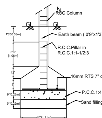
FOUNDATION DETAILS
