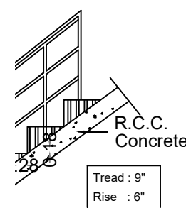
STAIRCASE DETAILS
