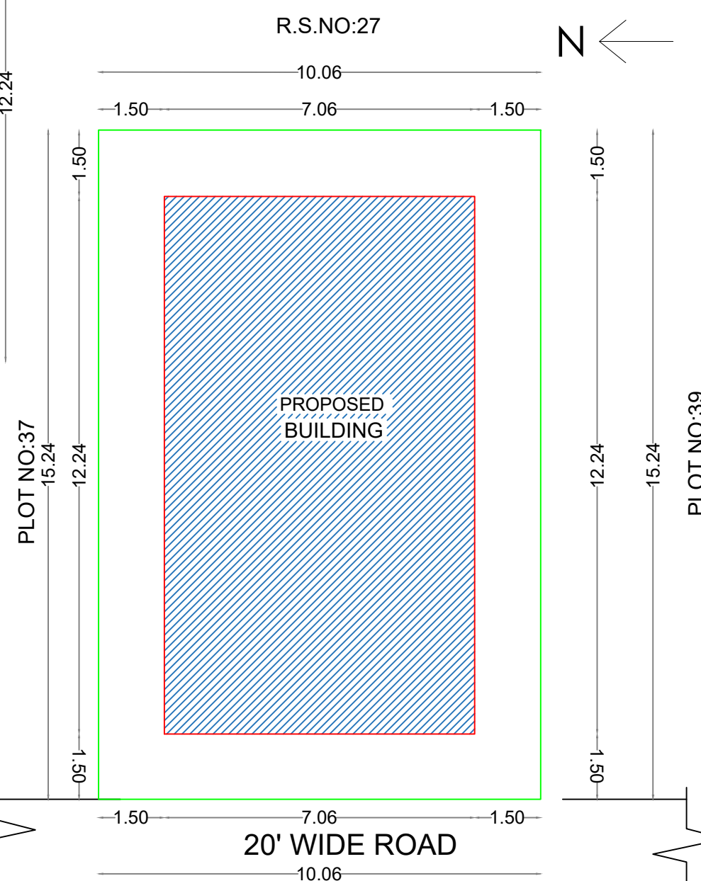
SITE PLAN
