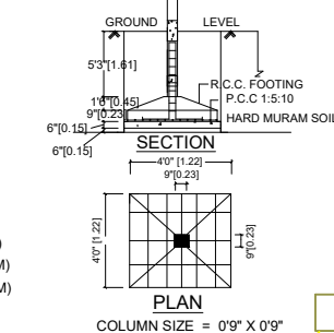
FOUNDATION DETAILS
