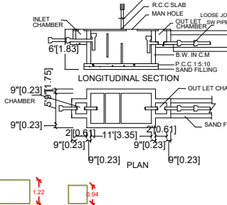
SEPTIC TANK:
