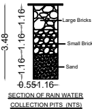
SECTION OF RAIN WATER COLLECTION PITS (NTS)
