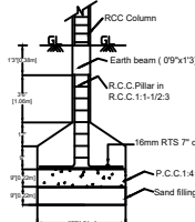
FOUNDATION DETAILS
