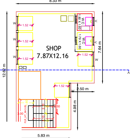
POSED FIRST FLOOR PLAN
