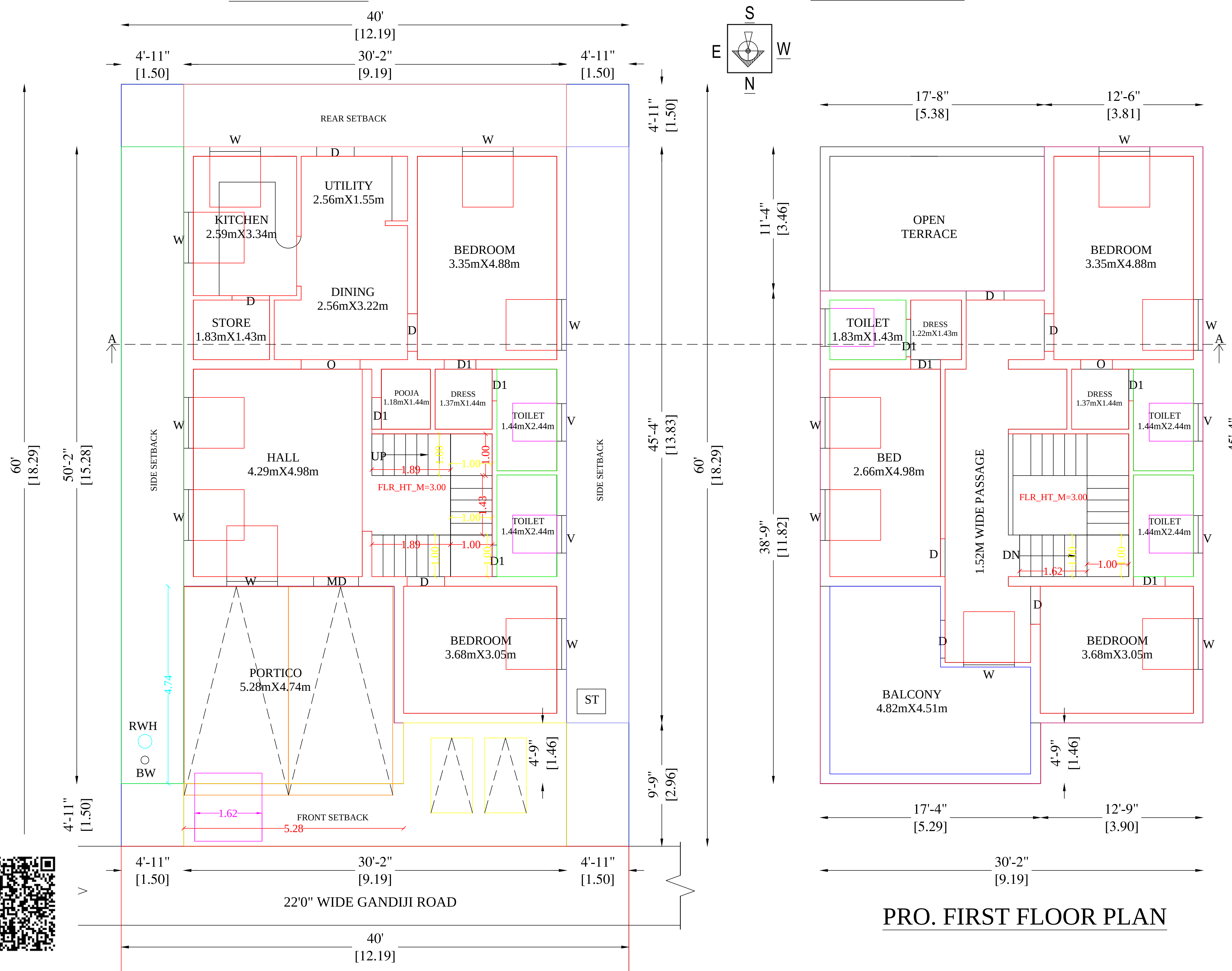
PRO. GROUND FLOOR PLAN
