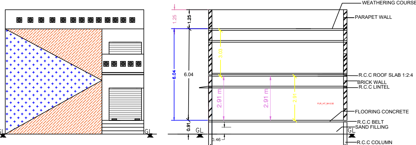
FRONT ELEVATION
