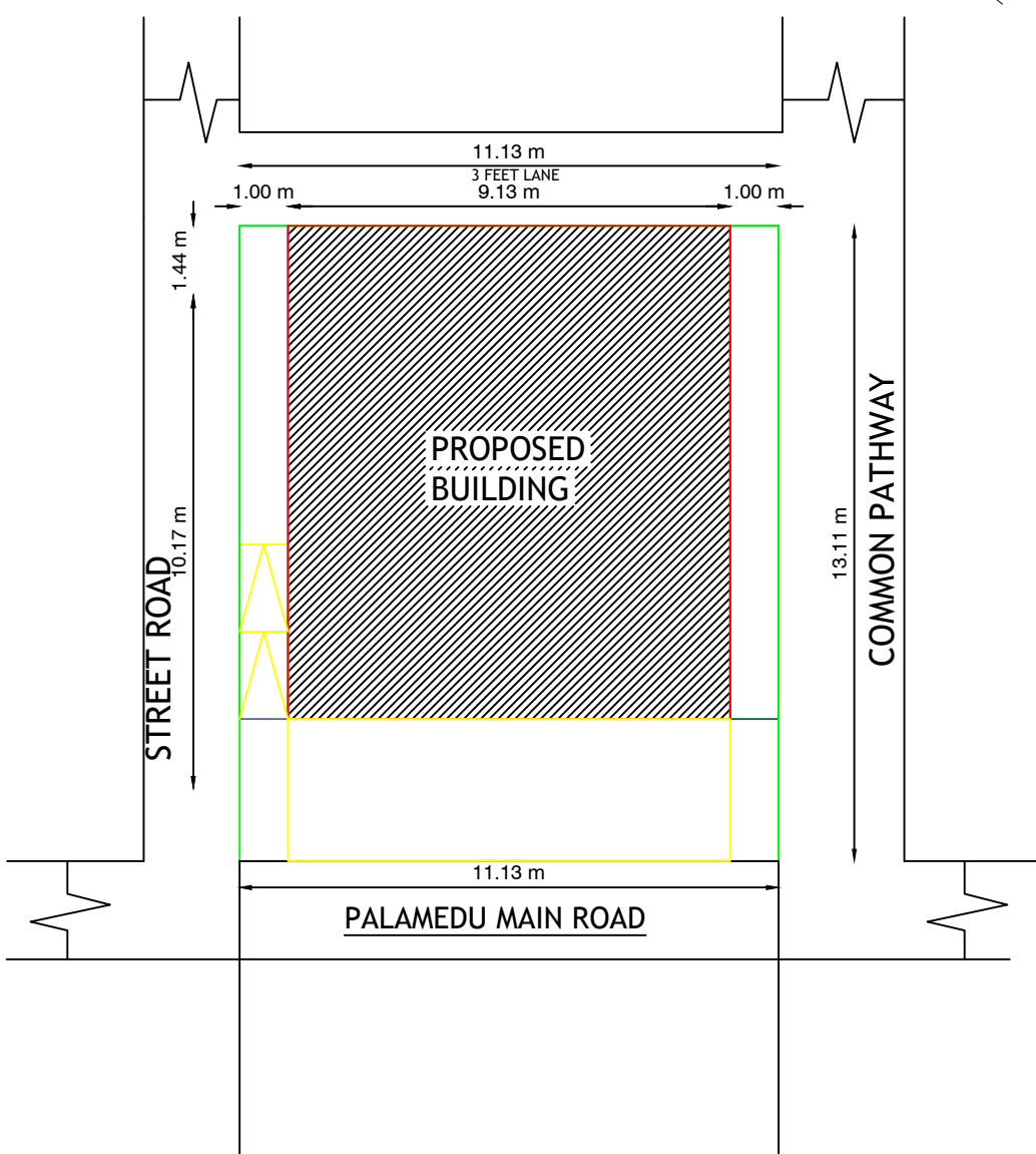
SITE PLAN
