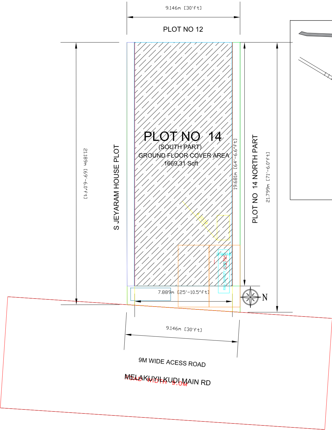
SITE LAYOUT PLAN
