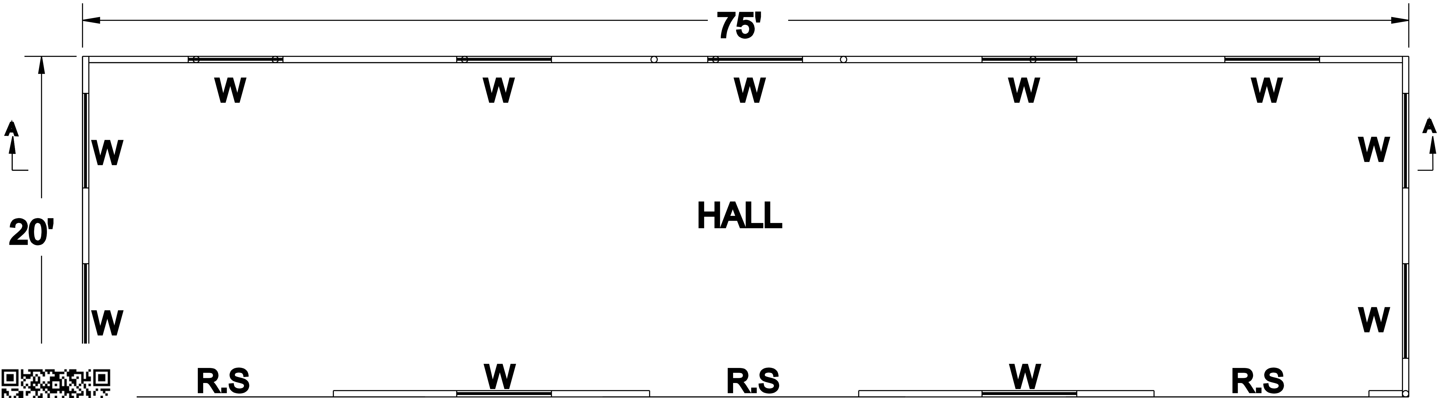
G.F. PLAN
