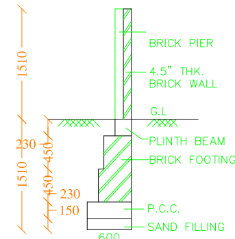
SCALE : 1" = 100
