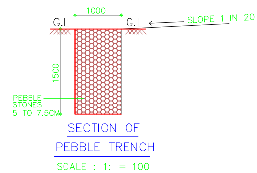
SCALE : 1" = 100
