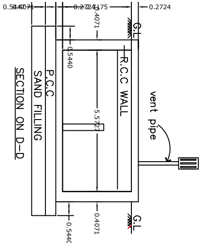
PLAN OF SEPTIC TANK SCALE 1"=2'0"
