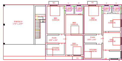
PROPOSED GROUND FLOOR PLAN
