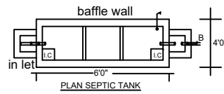
PLAN SEPTIC TANK
