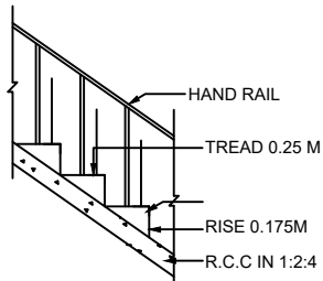
STAIRCASE DETAIL NOT TO SCALE
