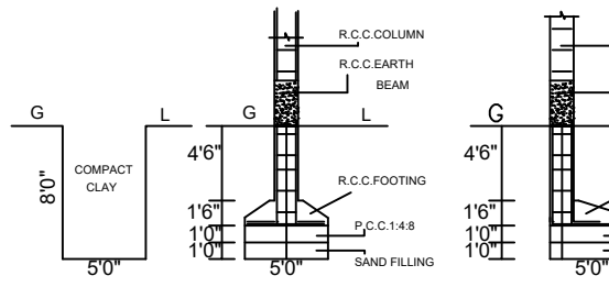
FOUNDATION DETAILS
