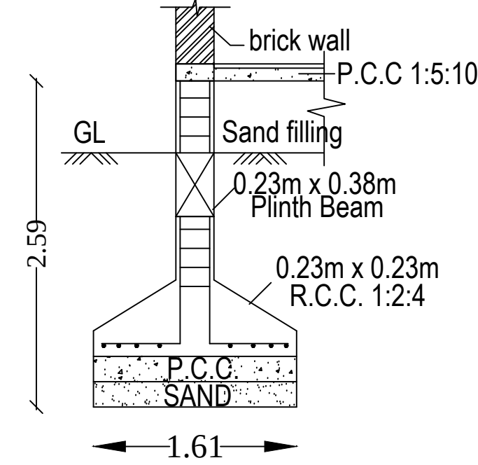
FOUNDATION DETAILS
