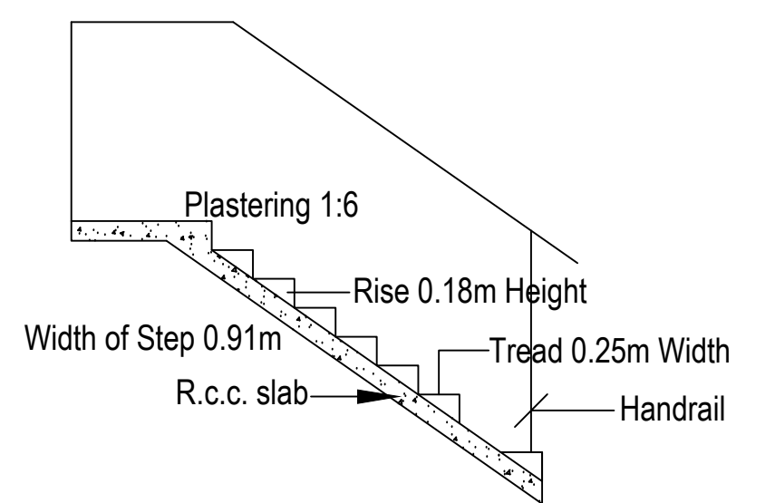
DETAILS OF STAIR CASE
