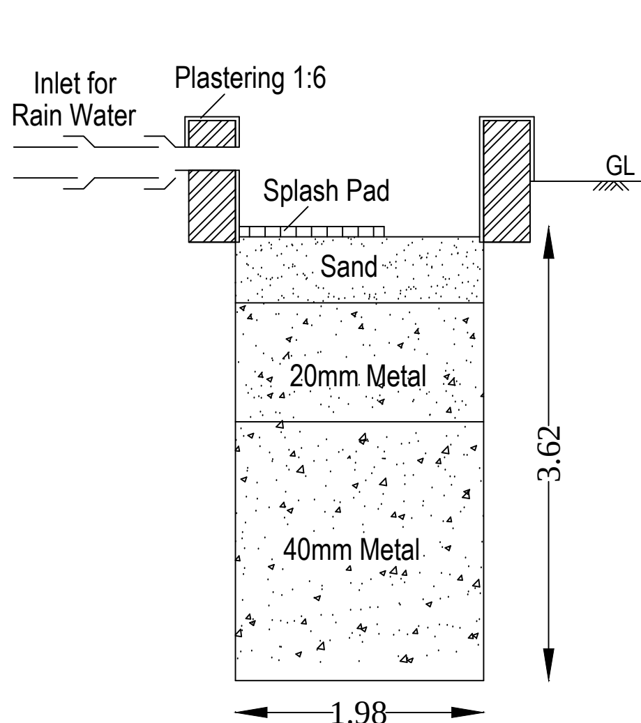
RAIN WATER PERCOLATION PIT
