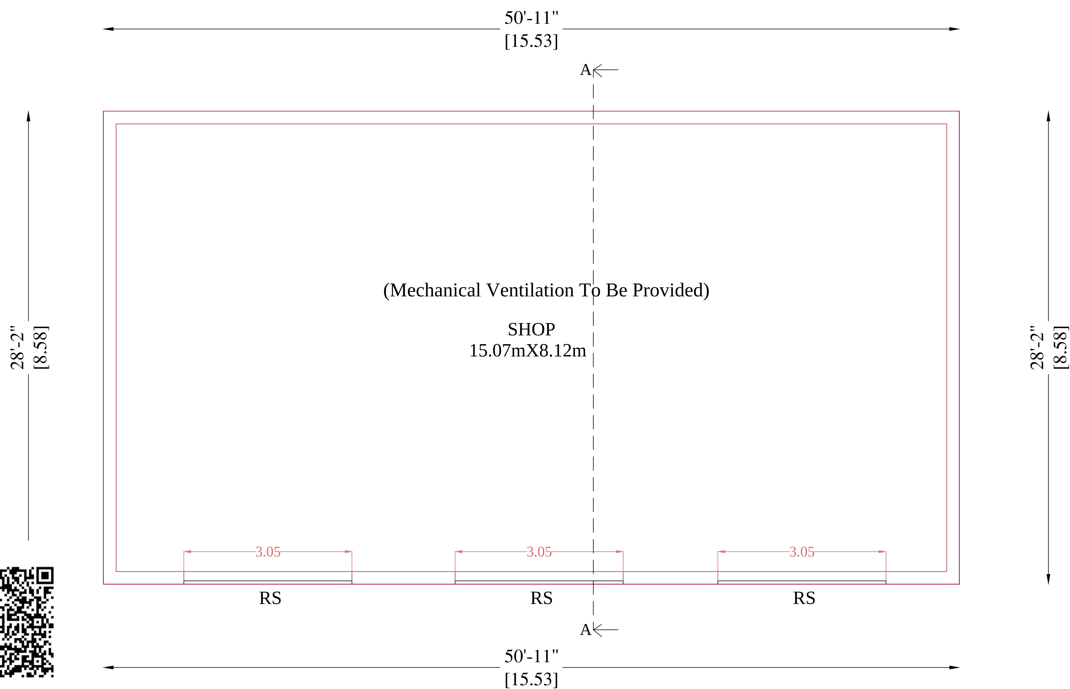
PRO. GROUND FLOOR PLAN
